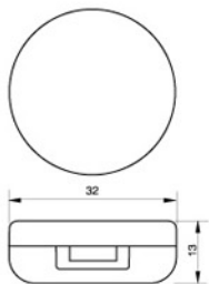
GLP M-20 • MAT'L : ABS, GLASS • 2g
