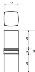
GLP PL-111 • MAT'L : ABS, PC
