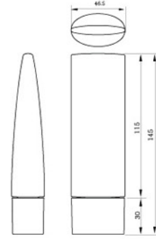
GLP ST-70 • MAT'L : ABS, PP, EVOH • 70ml
