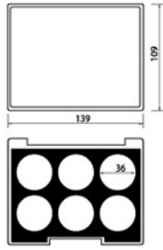
GLP PR-5 • MAT'L : ABS, EVA
