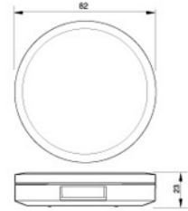
GLP M-1 • MAT'L : ABS, PC, GLASS • 15g / 18g / 20g
