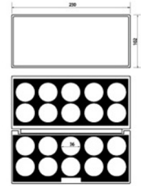
GLP PR-6 • MAT'L : ABS, EVA
