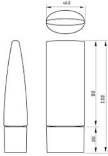
GLP ST-60 • MAT'L : ABS, PP, EVOH • 60ml
