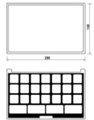
GLP PR-8 • MAT'L : ABS, EVA
