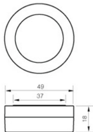
GLP M-3 • MAT'L : ABS, PC, PP • 5g
