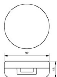
GLP M-20-1 • MAT'L : ABS, GLASS • 2g
